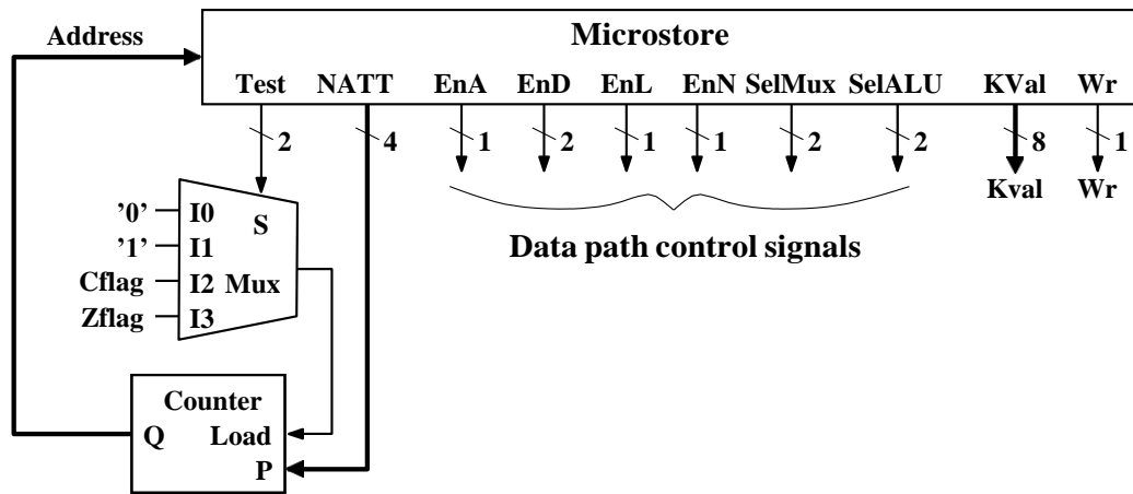
Figure 4: Microcode-Based Controller.
