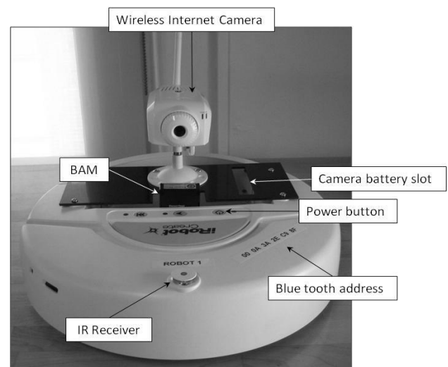
Figure 3: Modified iRobot Create Mobile Robot Platform.
