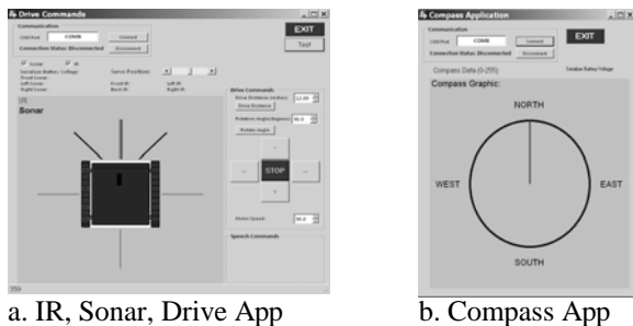
Figure 3: Visual C# GUI Screen shots.
