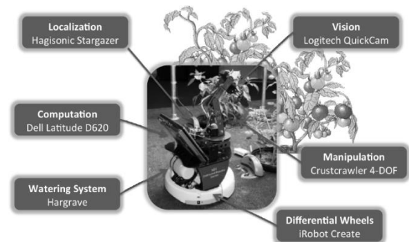
Figure 2: Robots are equipped with a 4-DOF end-effector, a monocular camera, an indoor, global localization system and watering device and are controlled by a notebook computer. Robots coordinate with each other and intelligent pots using wireless radio.
