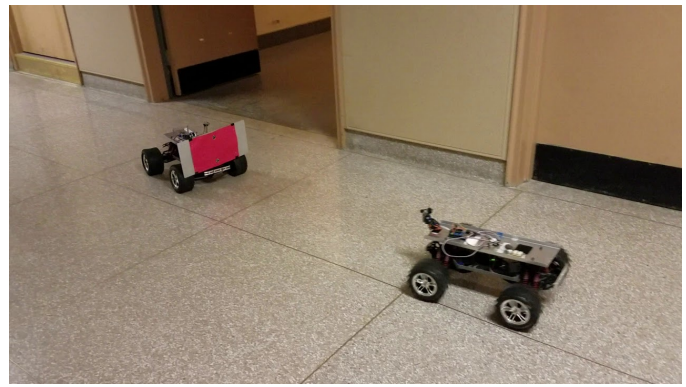
Fig. 3. Picture showing a pair of leader-follower robots in the hallway of our academic building. The camera mounted on the front of the follower vehicle is visible. The red paper on the leader is an easy-to-find target for computer vision.
