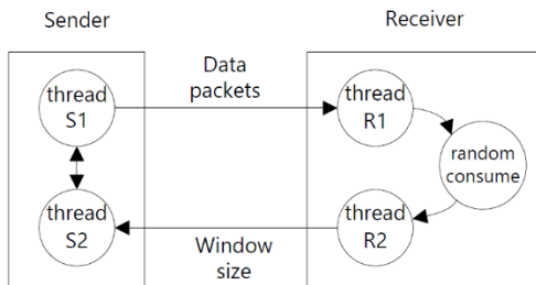
Figure 9: one Possible Flow Control Model in Multi-thread Mode
