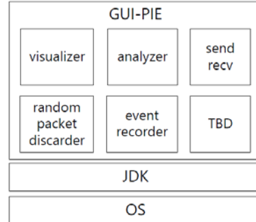
Figure 1: The Architecture of GUI-PIE
